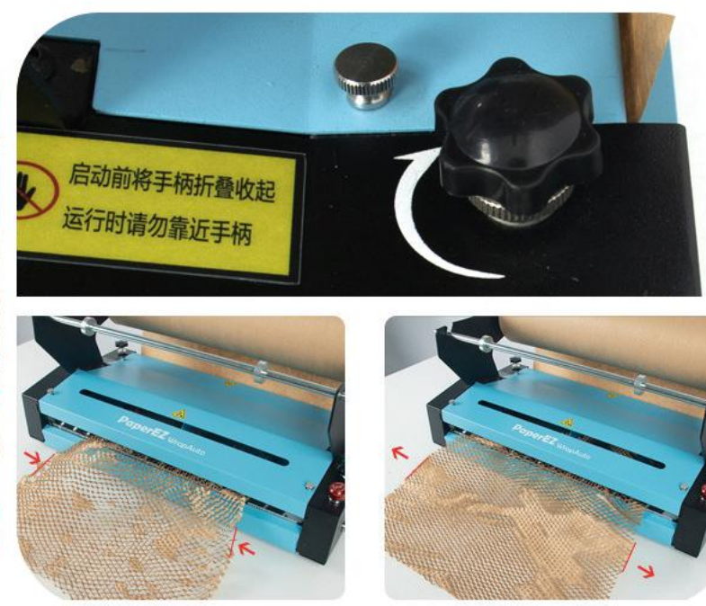
Tension Adjustable
